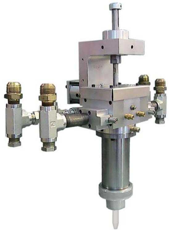
Dynamic Mixer with Recirculation (shown without motor)
